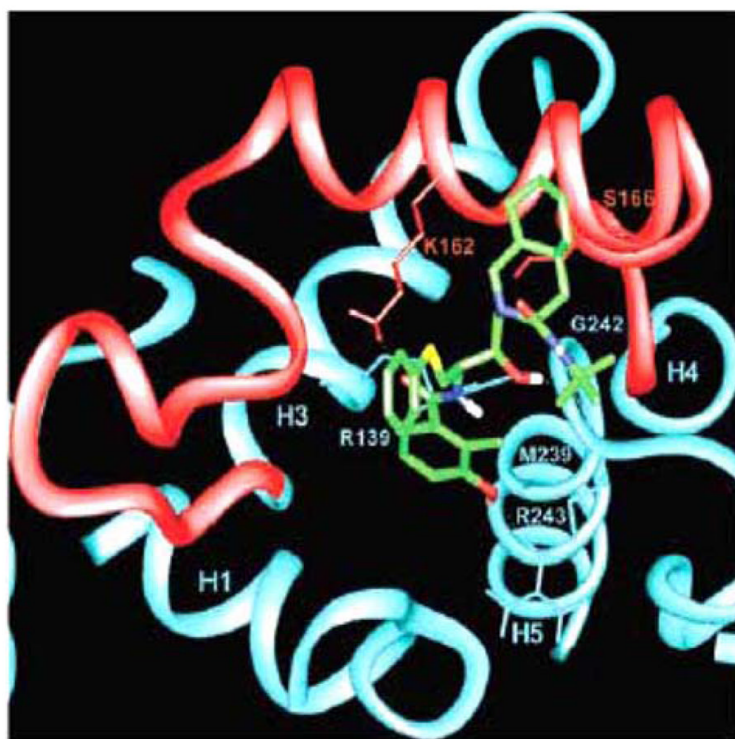
Fig. 1. Computer-simulated model of NFV (green) interaction with ANT (blue and red). Close-up of the proposed binding mode of NFV to the matrix side of ANT. Parts of helices 1, 3, 4, and 5 (H1, H3, H4, and H5) are shown. Loop M2, connecting helices 3 and 4, is shown in red. Hydrogen bonds are displayed as dotted lines.
